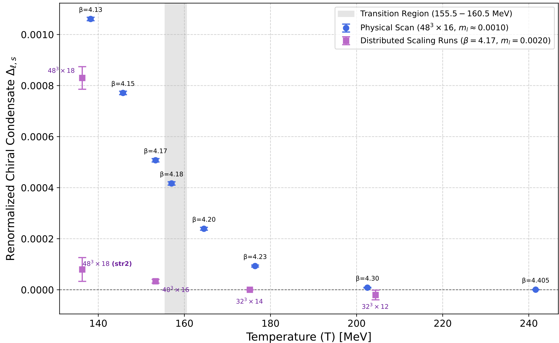
Global Chiral Condensate Evolution Across All 13 Ensembles
