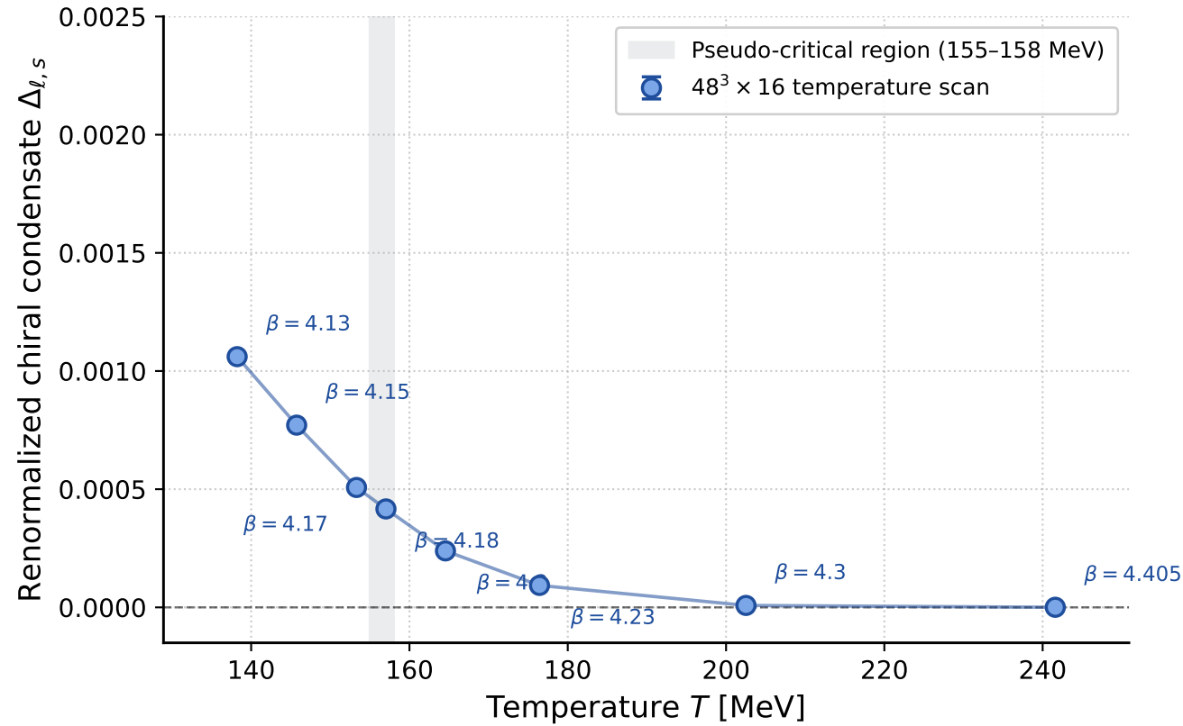
Series A — 48^3 \times 16 temperature scan ( \beta sweep)
