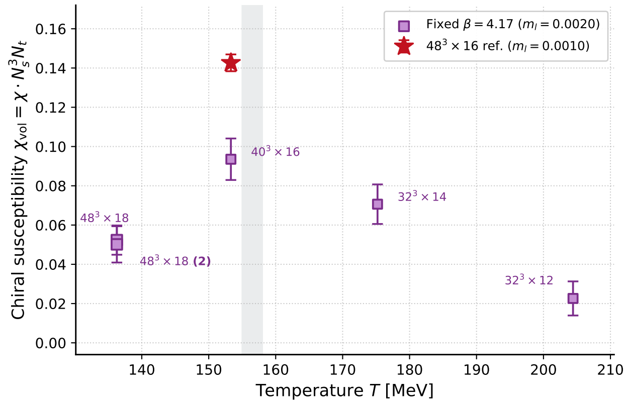
Series B — fixed \beta = 4.17 ( N_s/N_t variation)
