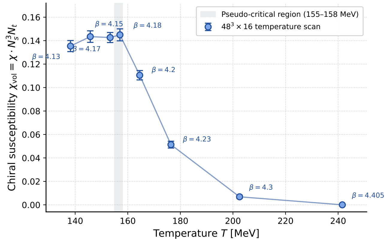
Series A — 48^3 \times 16 temperature scan ( \beta sweep)
