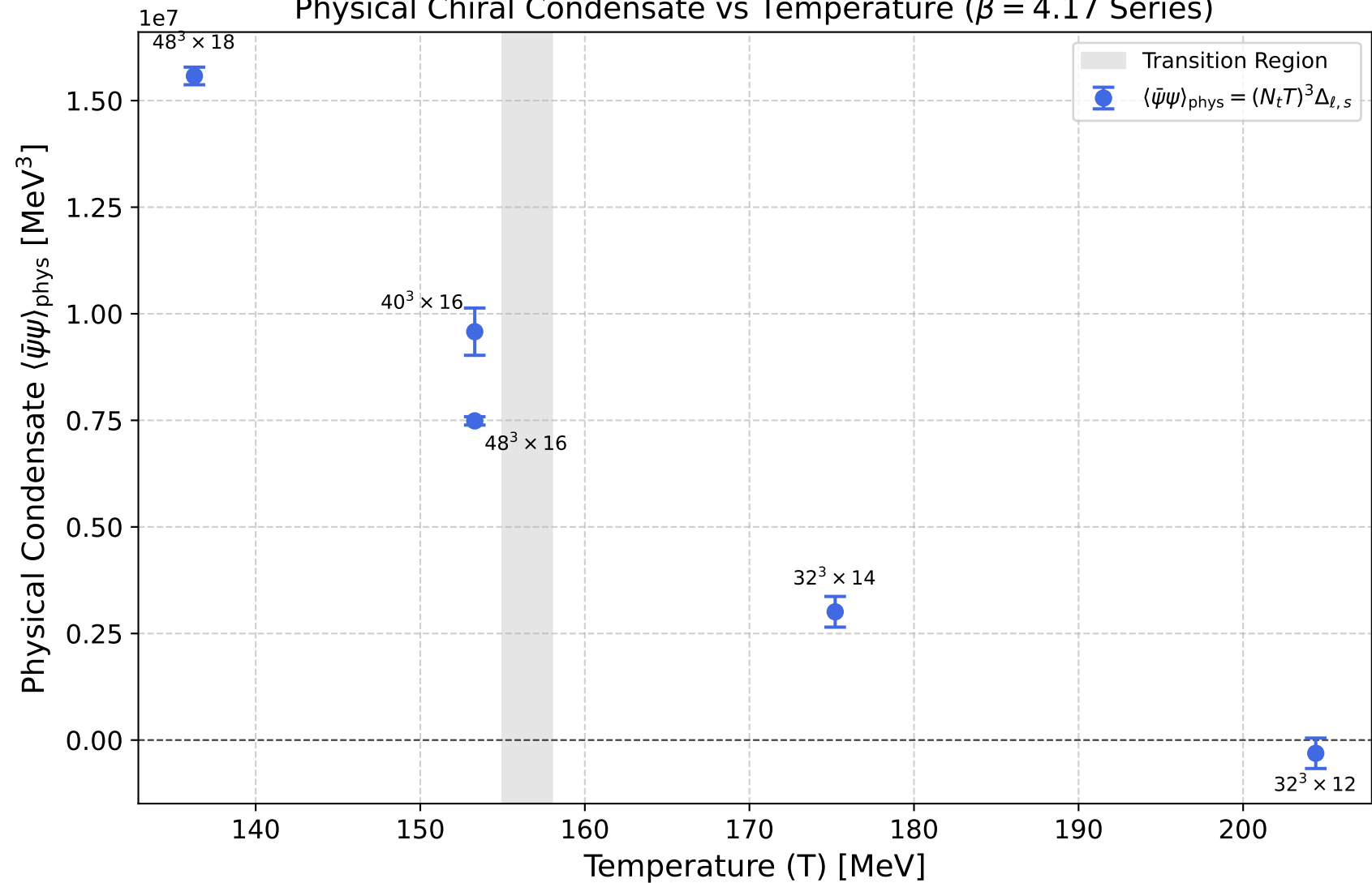
Physical Chiral Condensate vs Temperature ( \beta = 4.17 Series)
