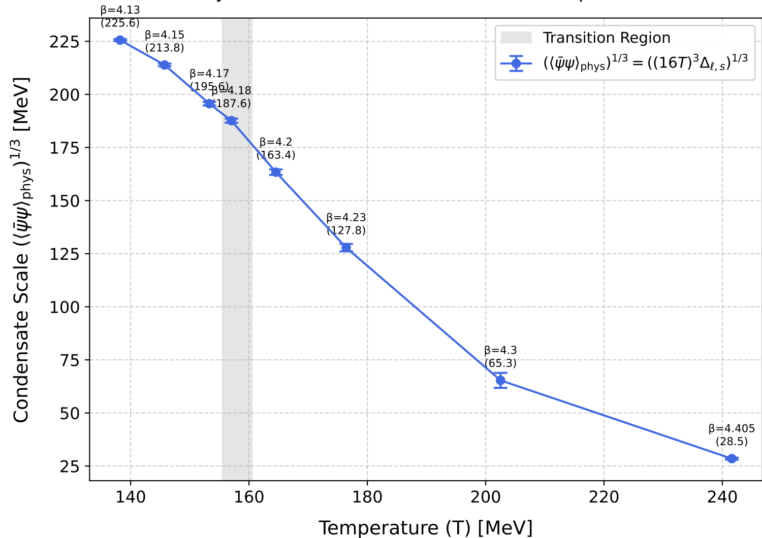
Physical Chiral Condensate Scale vs Temperature
