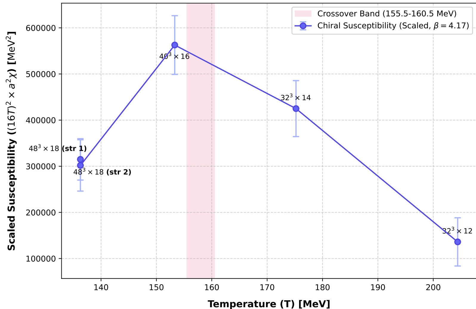
Chiral Susceptibility vs Temperature (Scaled)
