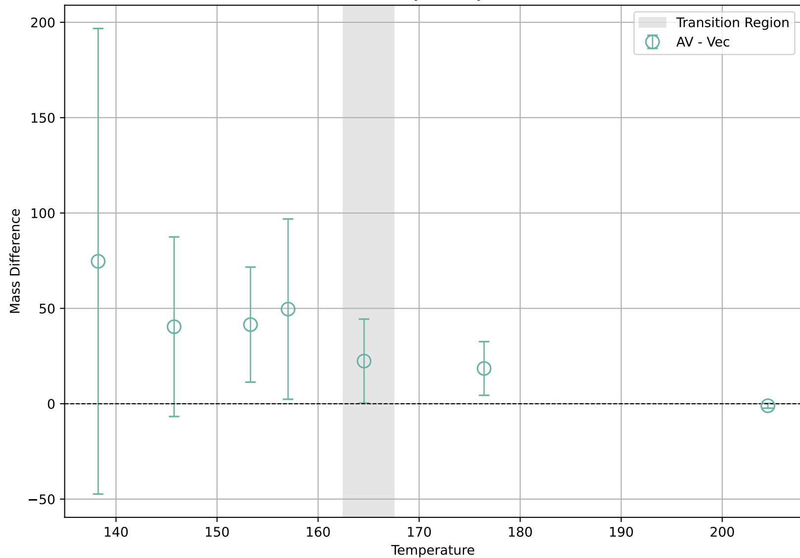
Chiral Flavor Symmetry (AV - Vec)
