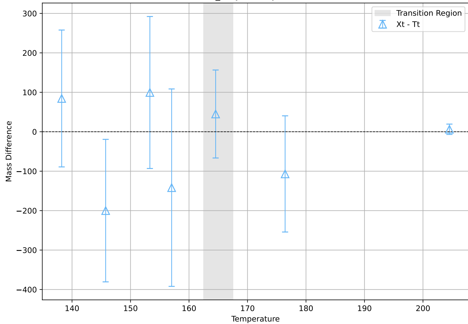
U(1)_A Symmetry ( X_t - T_t )
