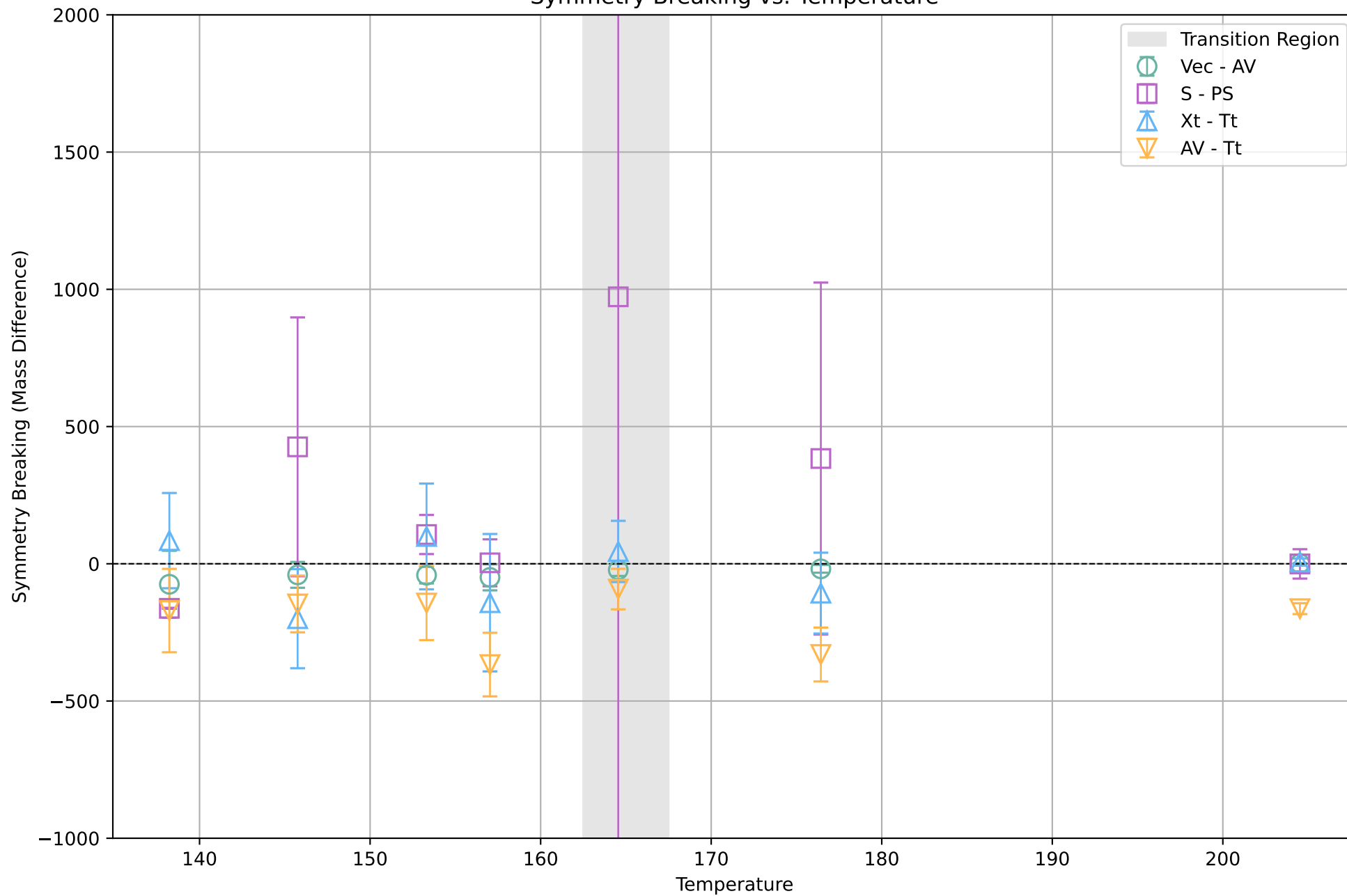
Symmetry Breaking vs. Temperature
