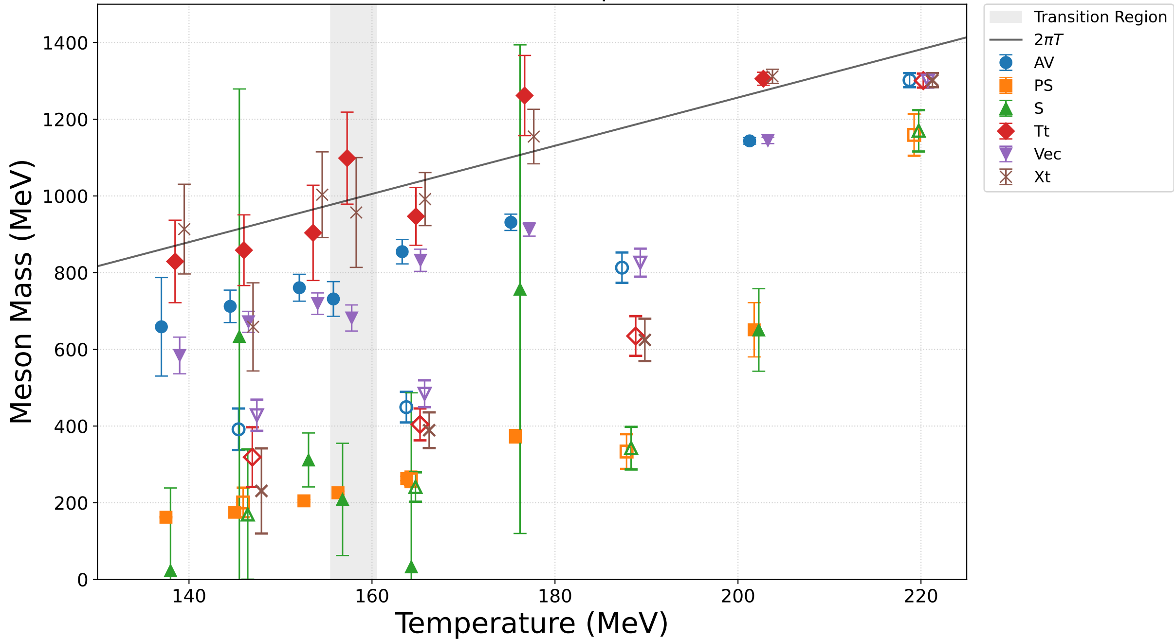
Meson Mass vs. Temperature
