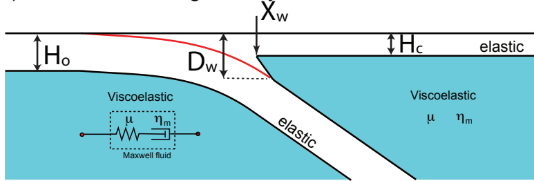
(c) interseismic coupling (steady flow)
