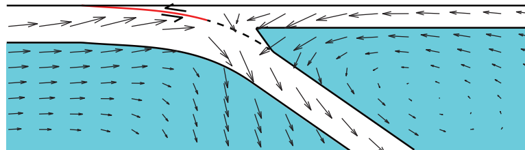
(d) repeated earthquakes (transient flow)
