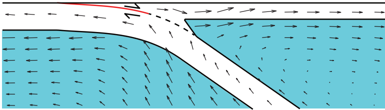
(c) interseismic coupling (steady flow)
