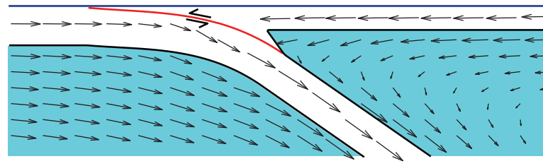
(d) repeated earthquakes (transient flow)
