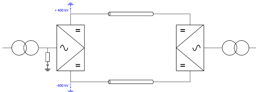
Figure 5: Symmetrical monopole (SMP) configuration.
