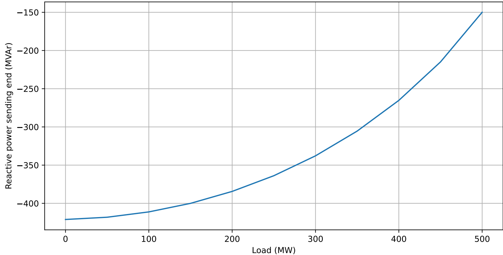
Reactive Power vs Load
