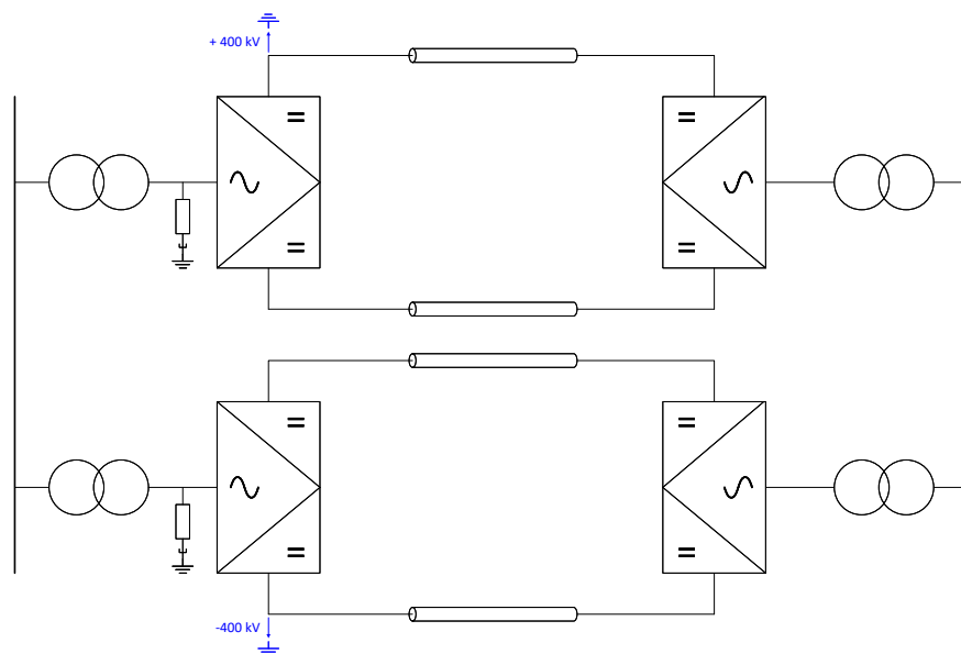
Figure 3: Dual symmetrical monopole (DSMP) configuration.
