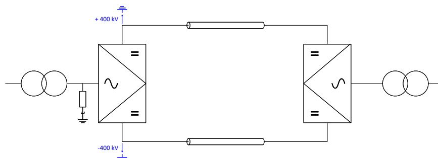
Figure 5: Symmetrical monopole (SMP) configuration.
