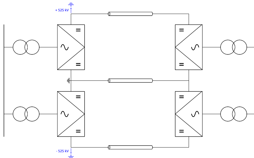
Figure 4: Bipole with dedicated metallic return (BIP) configuration.
