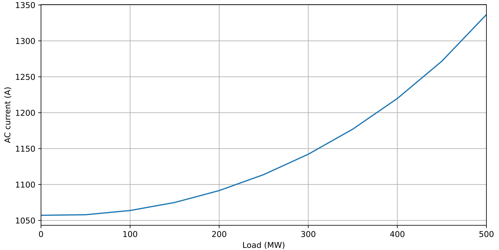
Current vs Load
