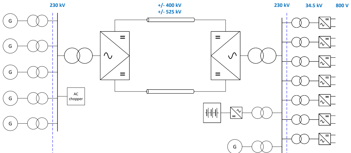
Figure 2: System overview with HVDC system scope of supply
