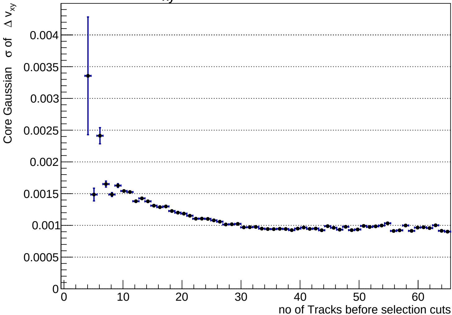
\Delta v_{xy} vs nwocutsTracks
