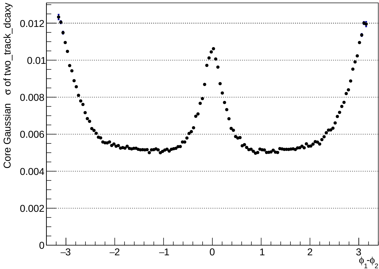
Two_track_phi_dcaxy
