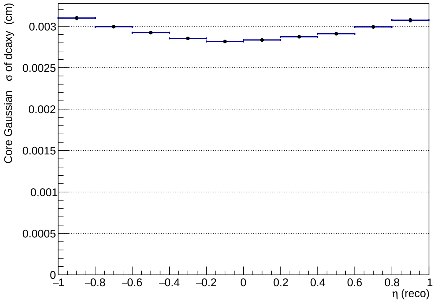
hdcaxy_vs_eta reco
