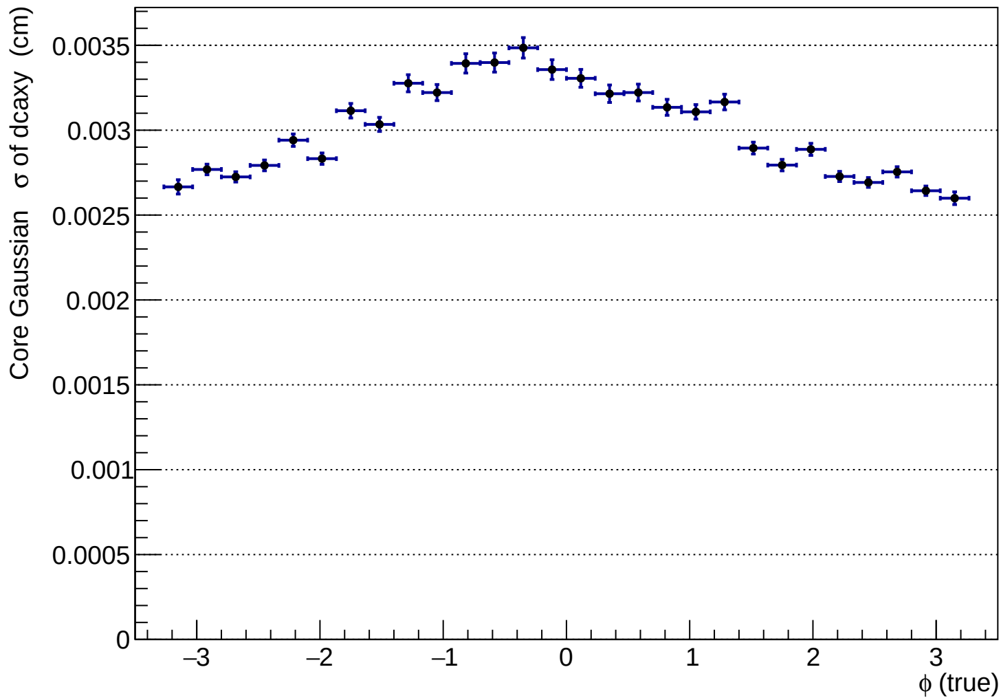
hdcaxy_vs_phitru_pi-
