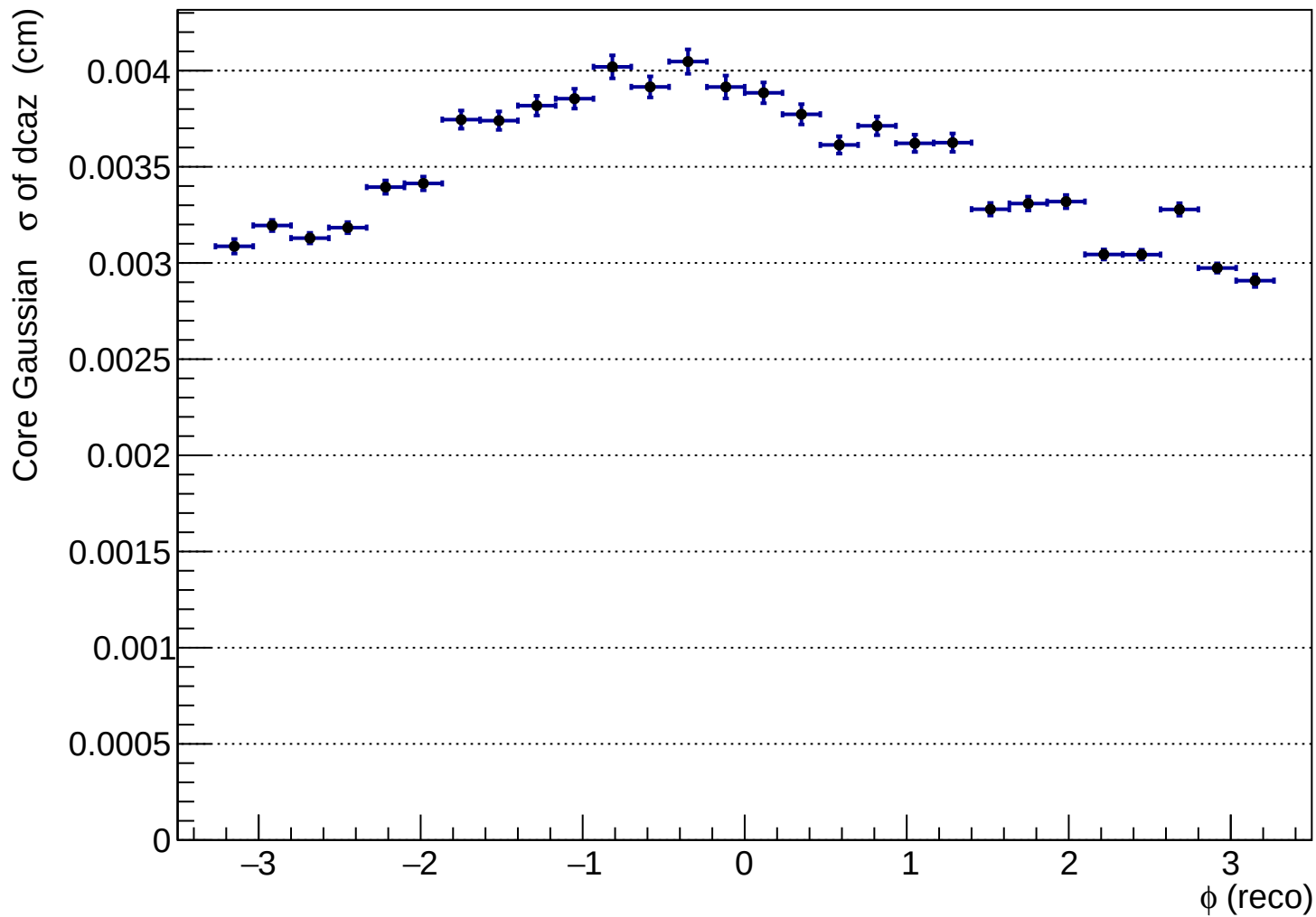
hdcaz_vs_phireco
