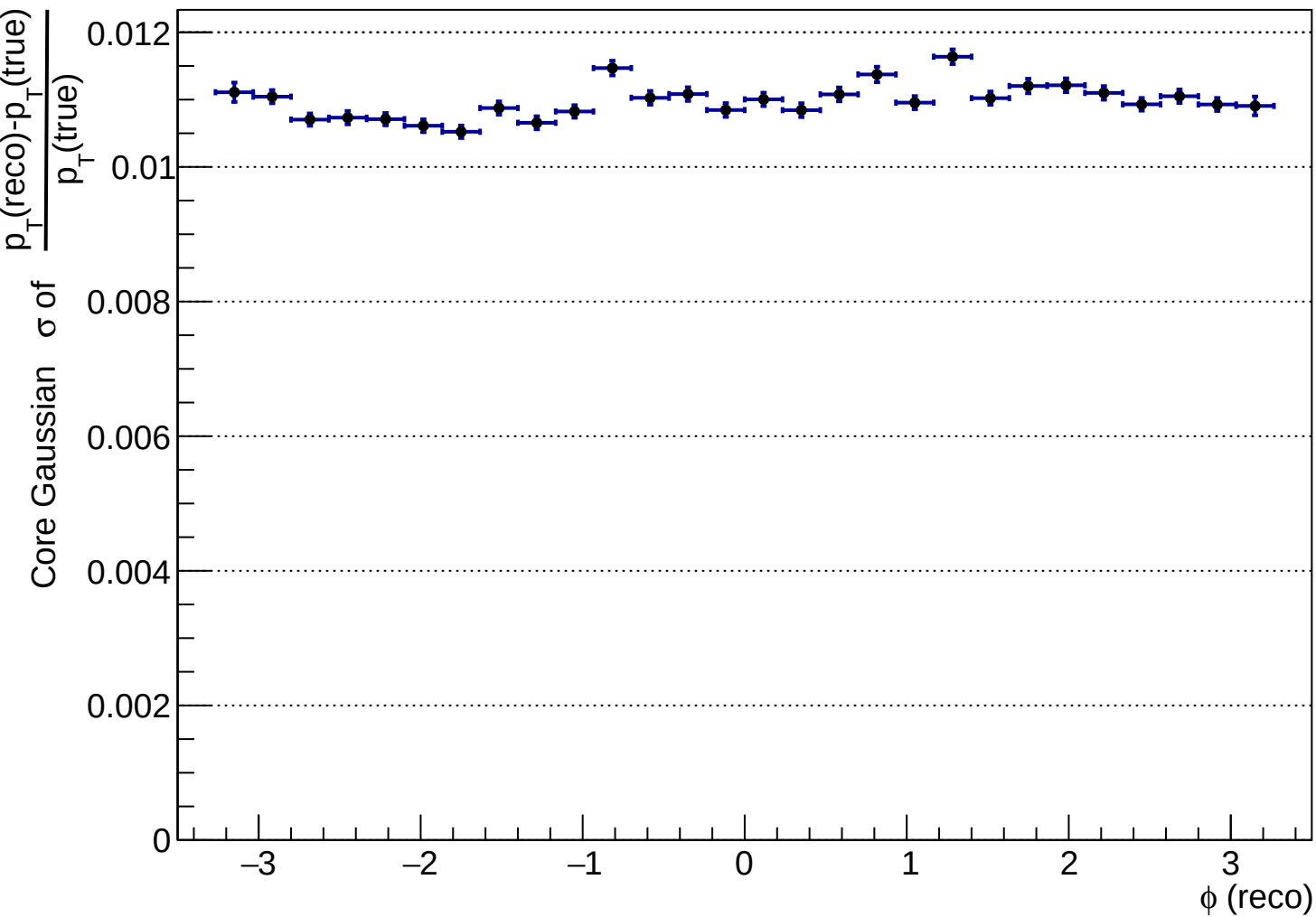
hptRes_vs_phireco_pi-
