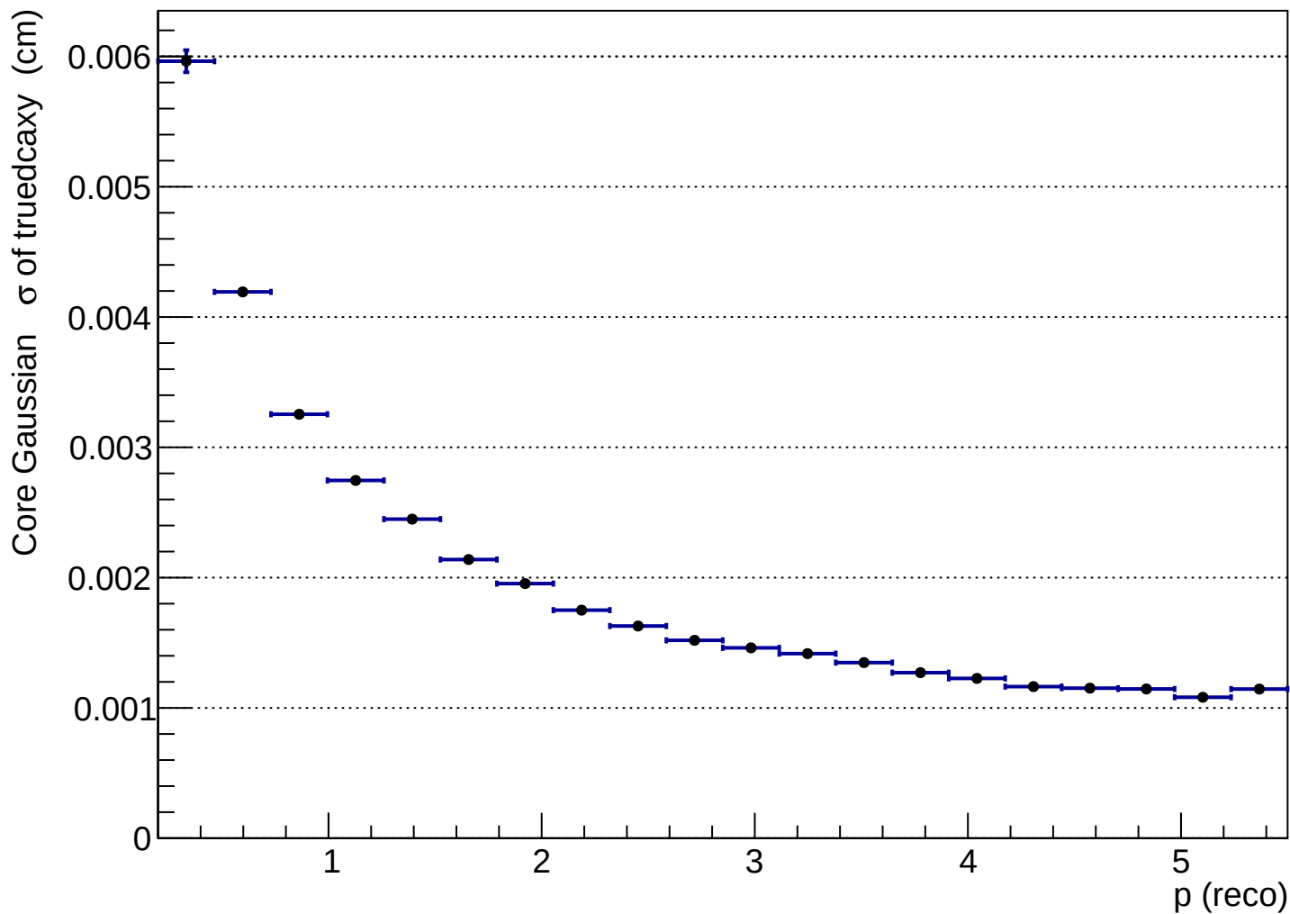
htruedcaxy_vs_preco
