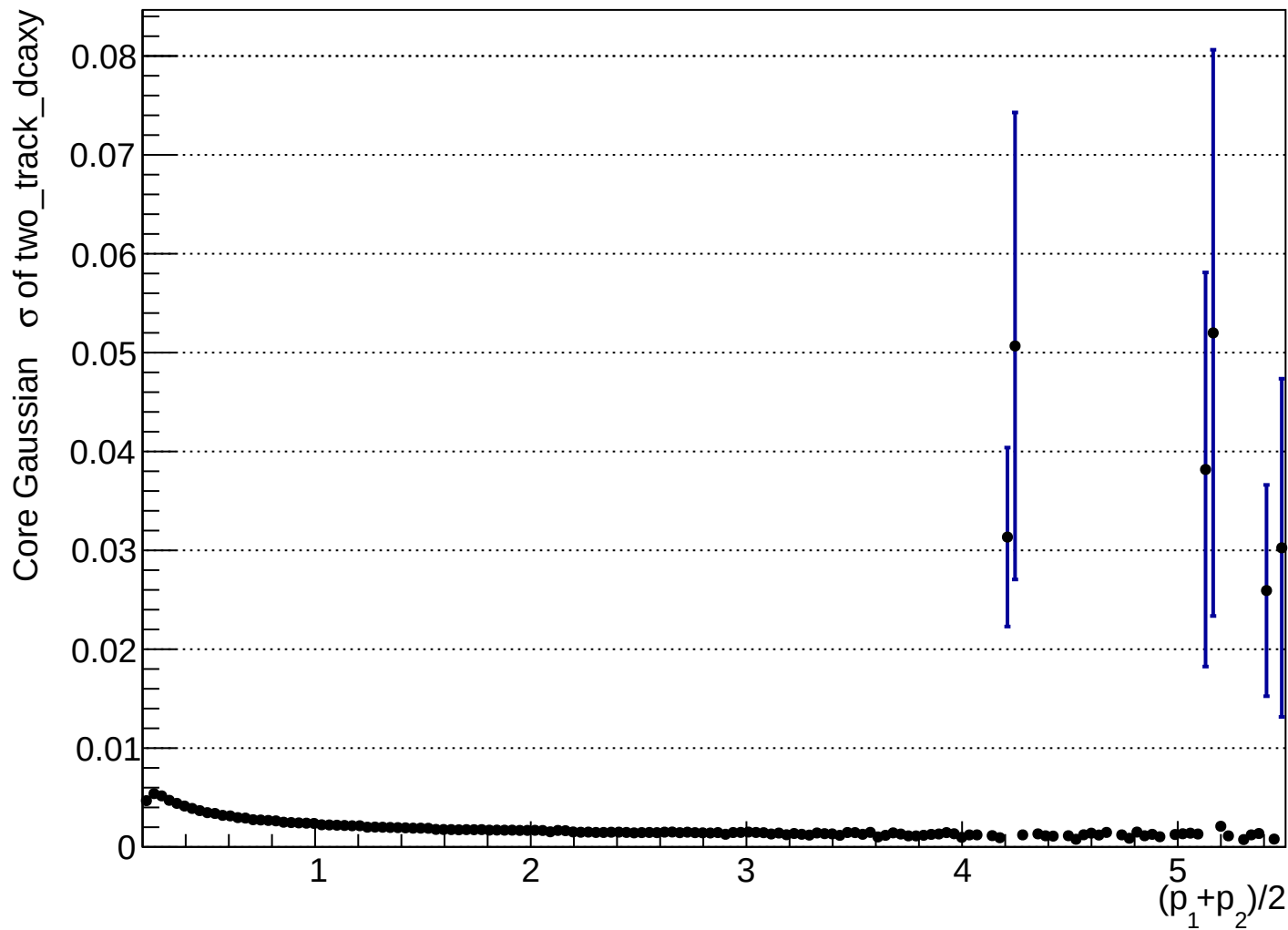
Two track dcaxy vs p
