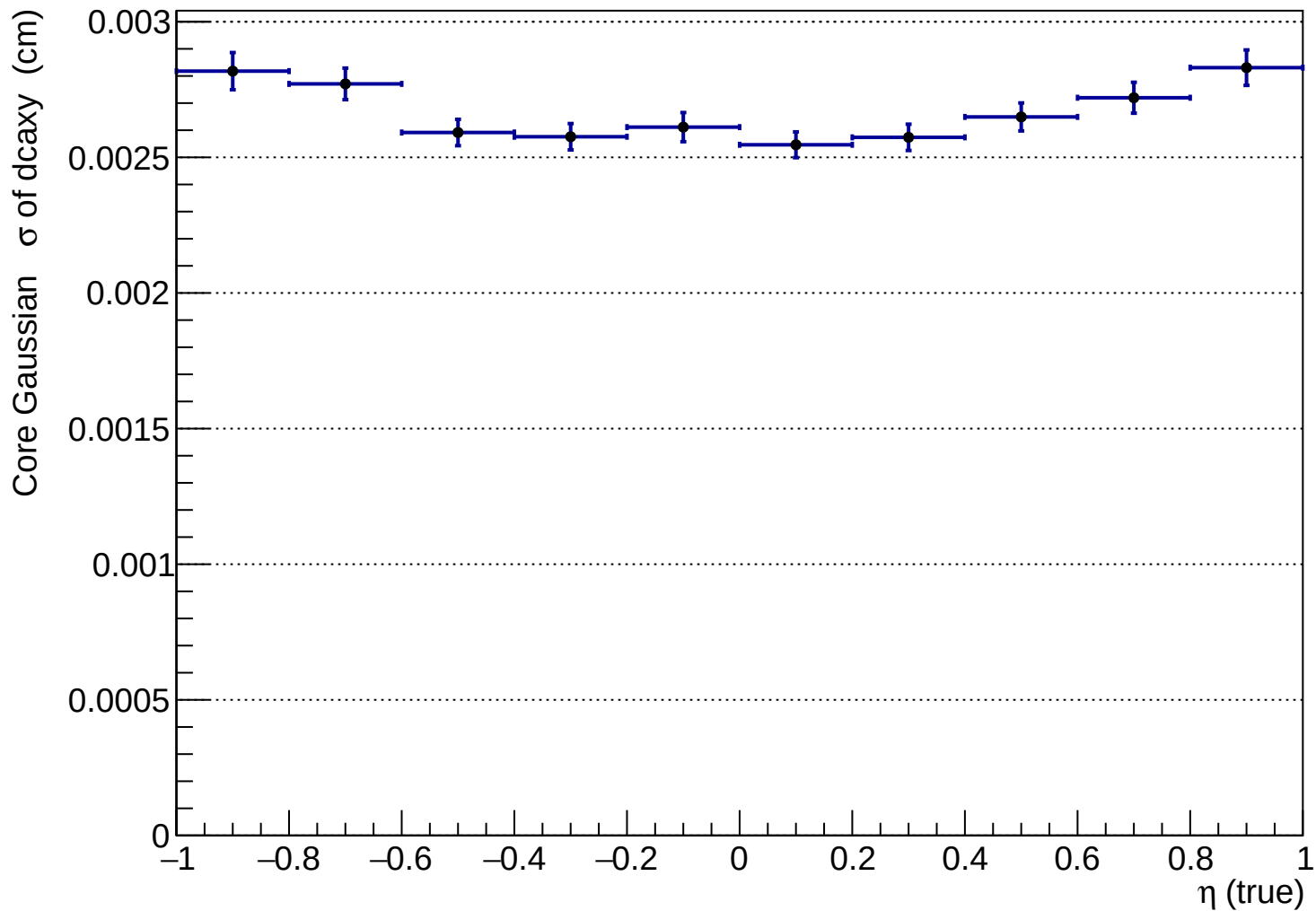
hdcaxy_vs_etatru_K-
