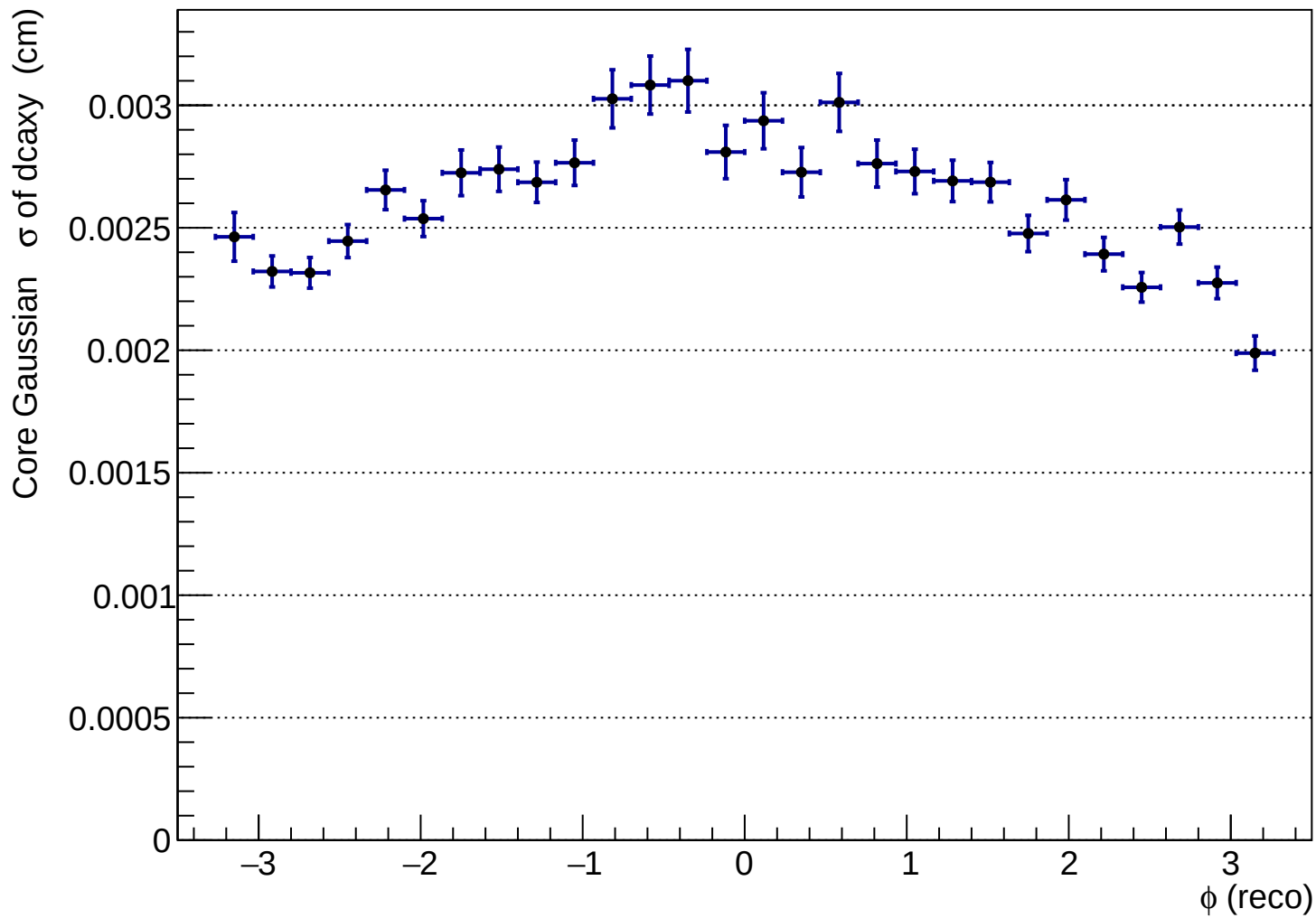
hdcaxy_vs_phireco_K+
