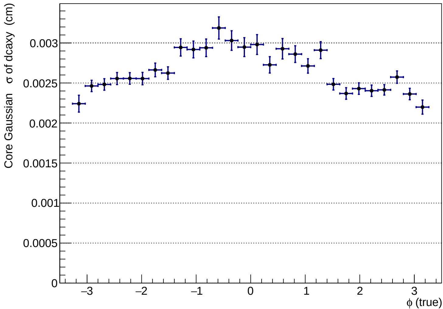
hdcaxy_vs_phitruue_K-
