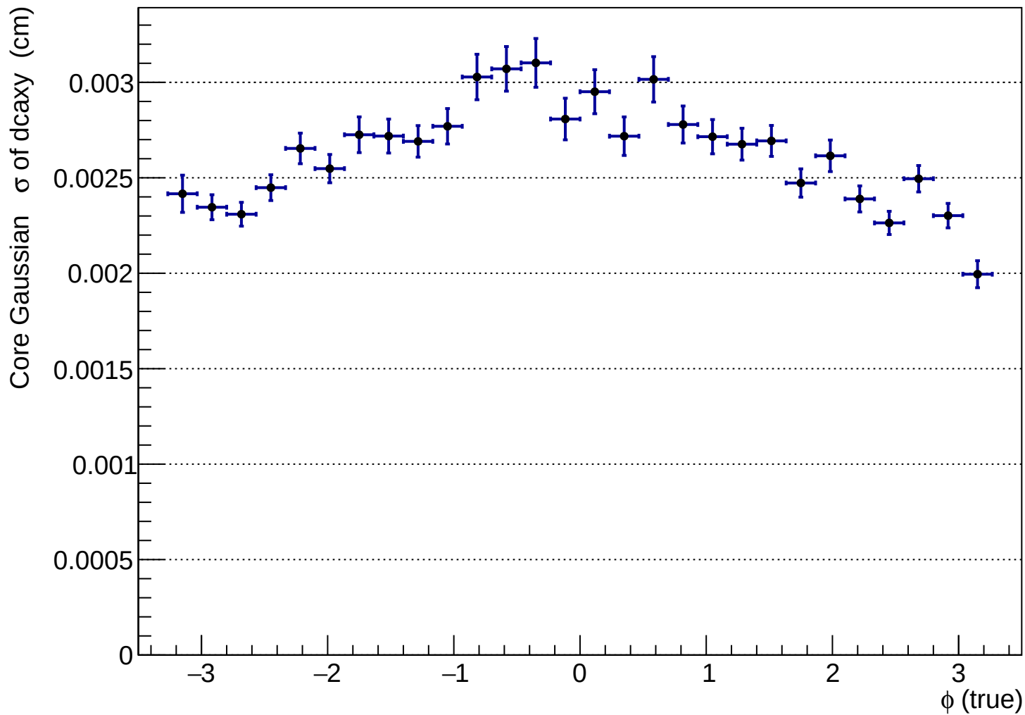
hdcaxy_vs_phitru_K+
