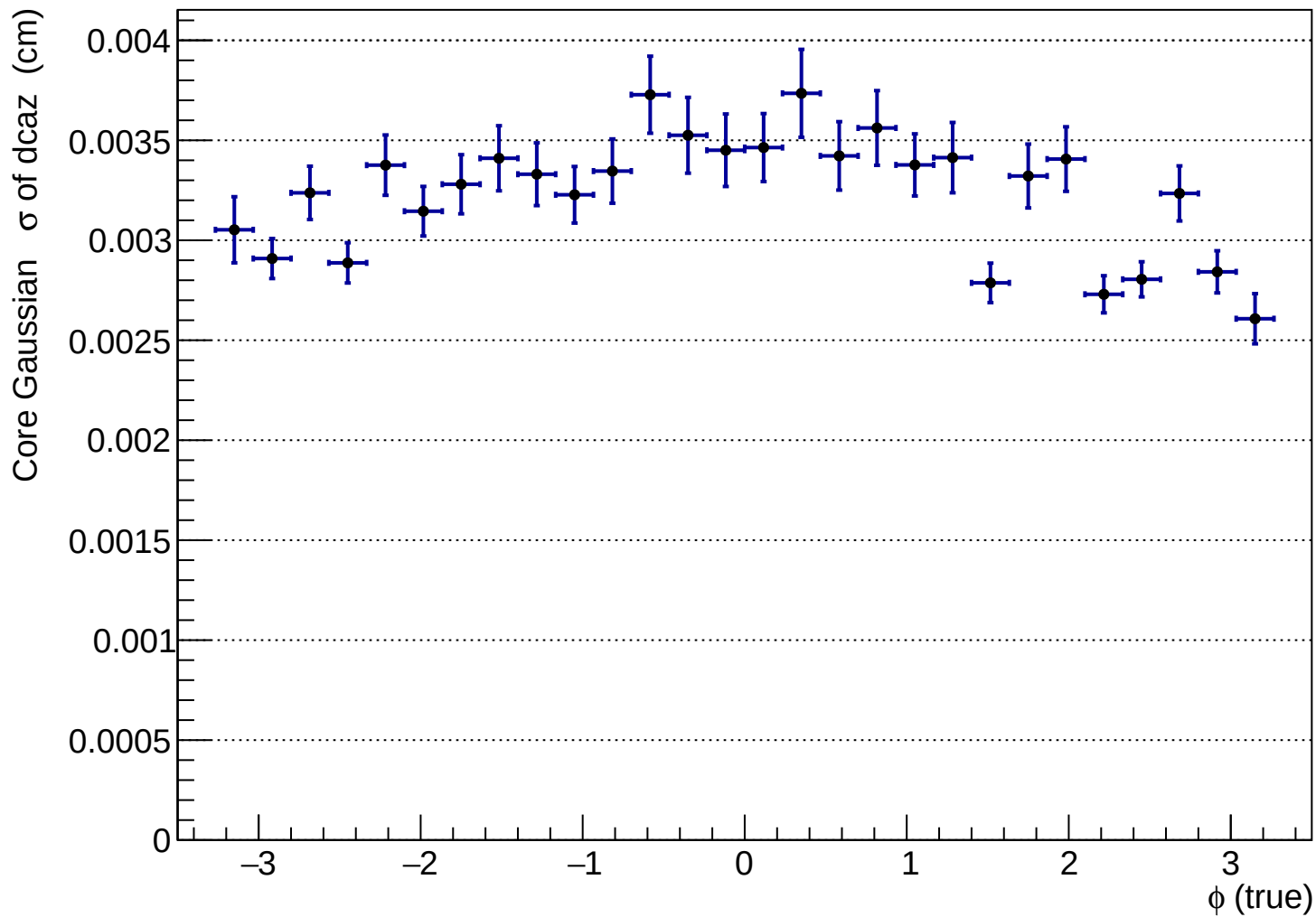
hdcaz_vs_phitru_K+
