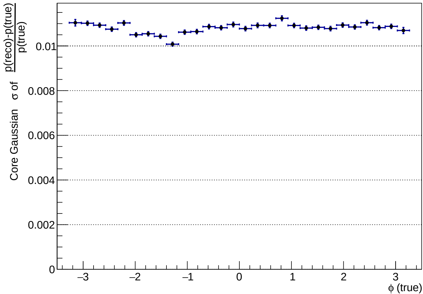
hpRes_vs_phitruue_pi+
