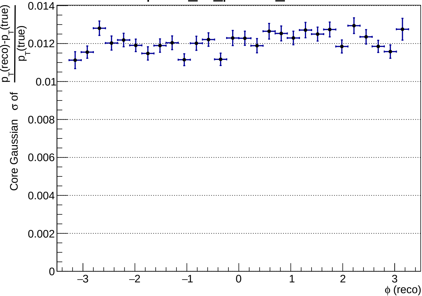
hptRes_vs_phireco_K-
