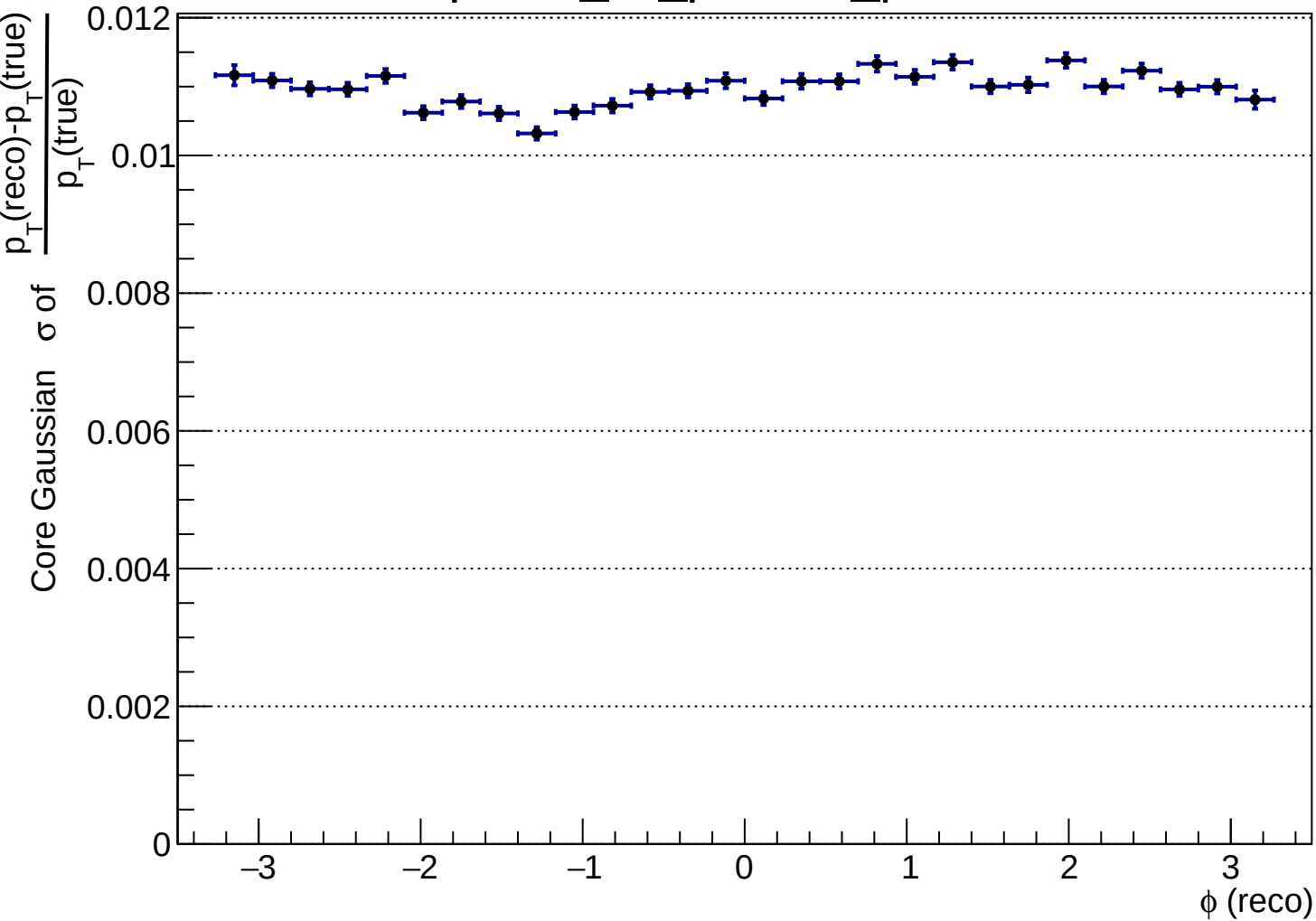
hptRes_vs_phireco_pi+
