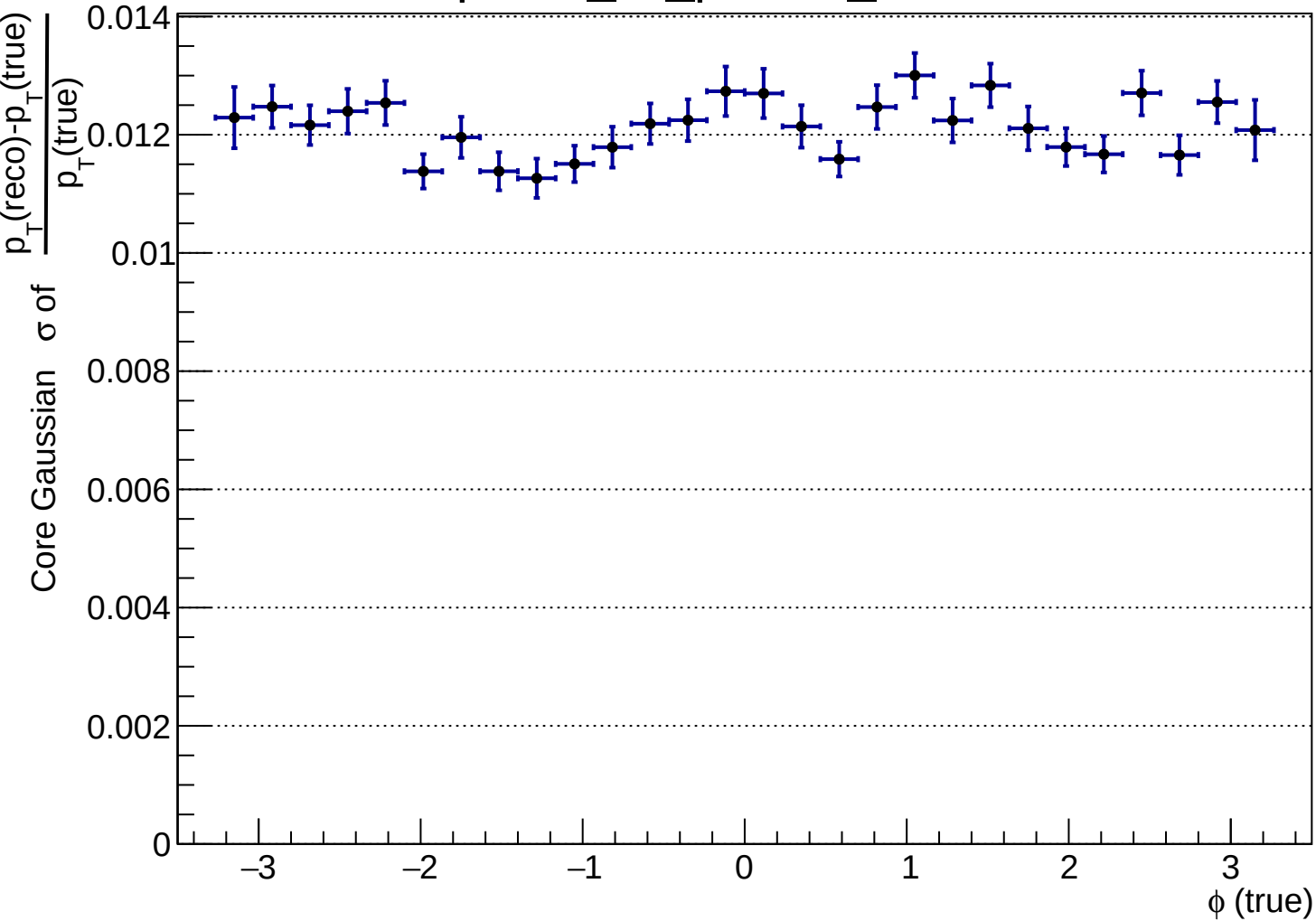
hptRes_vs_phittrue_K+
