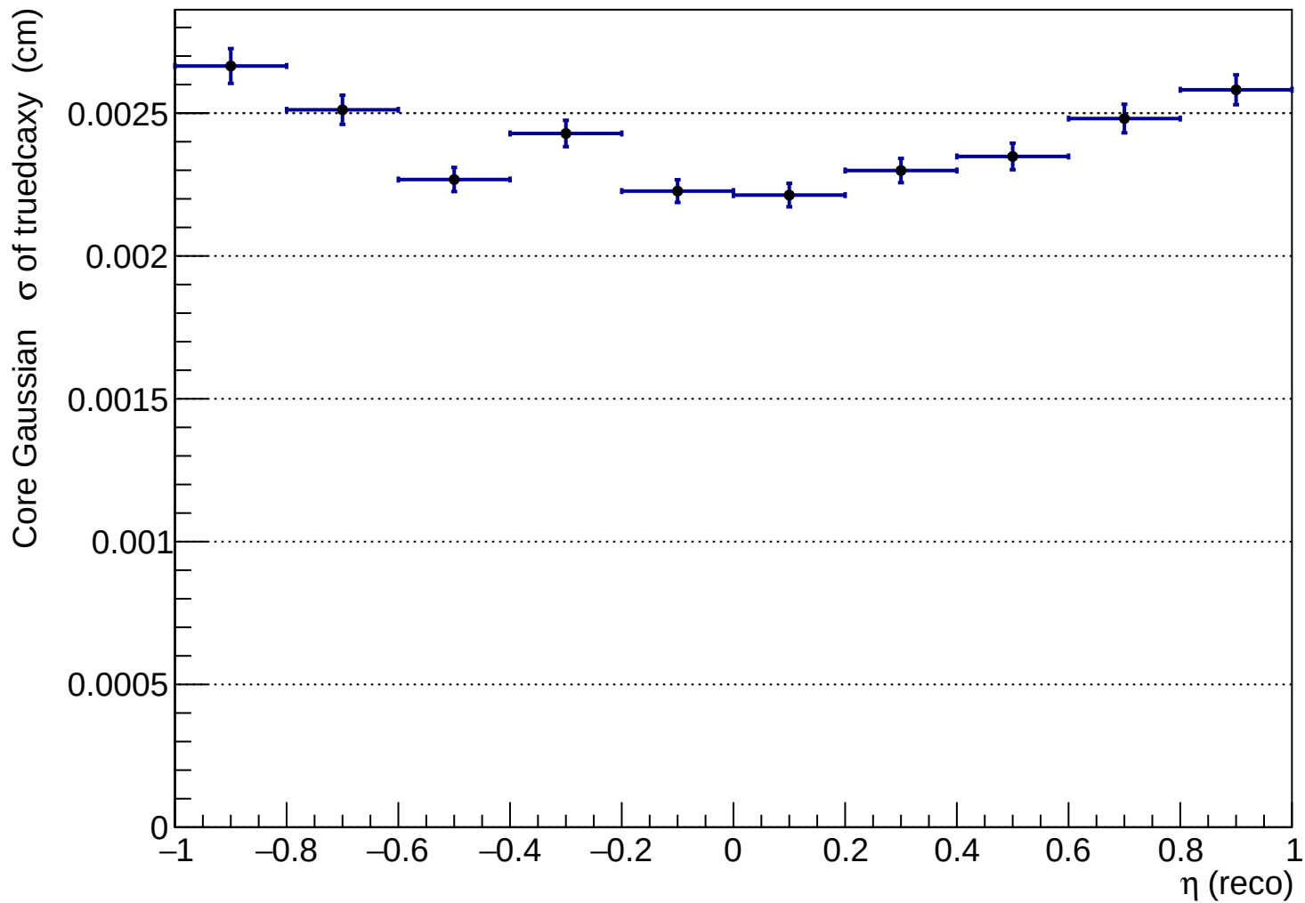
htruedcaxy_vs_eta reco_K+
