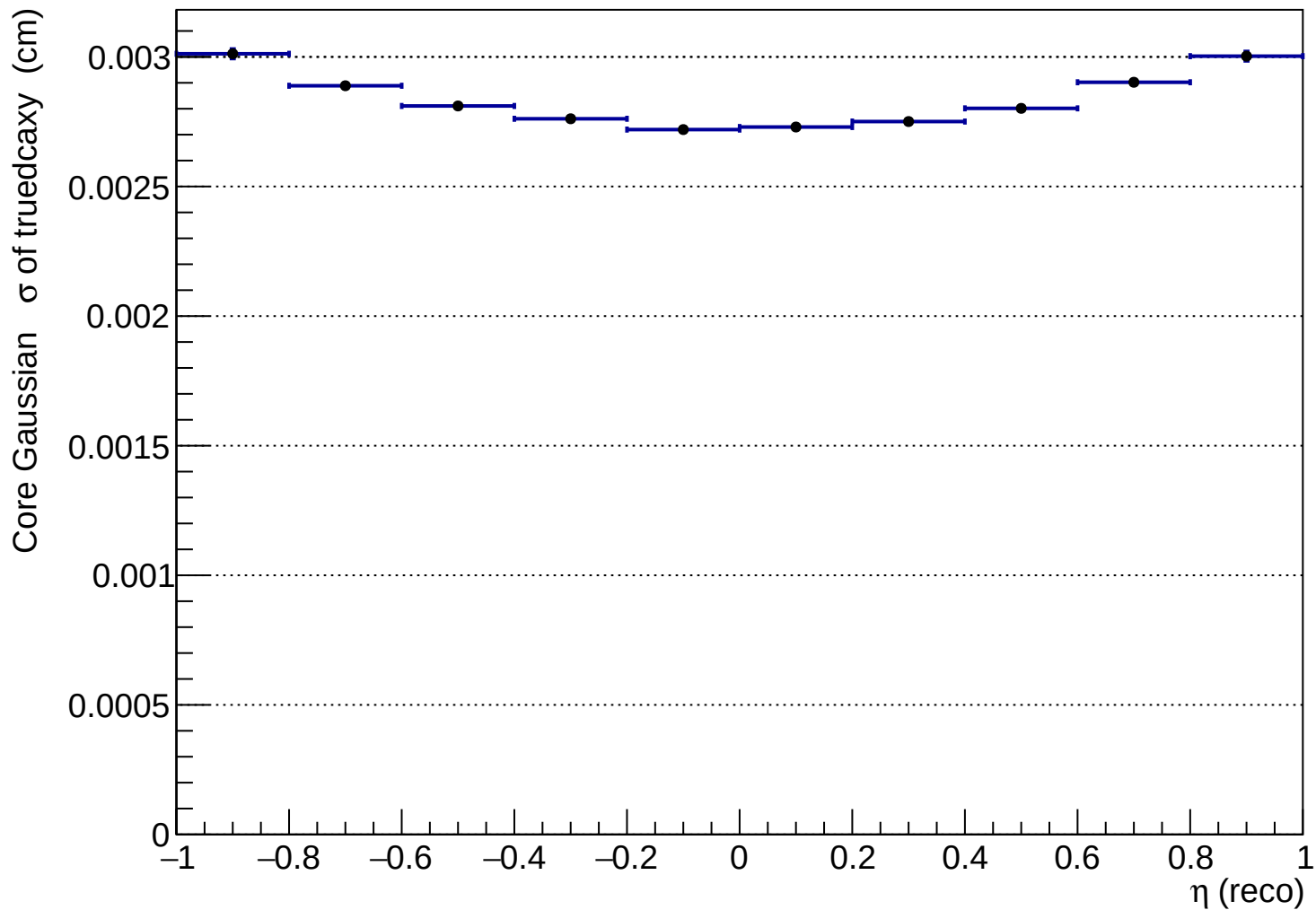
htruedcaxy_vs_eta reco
