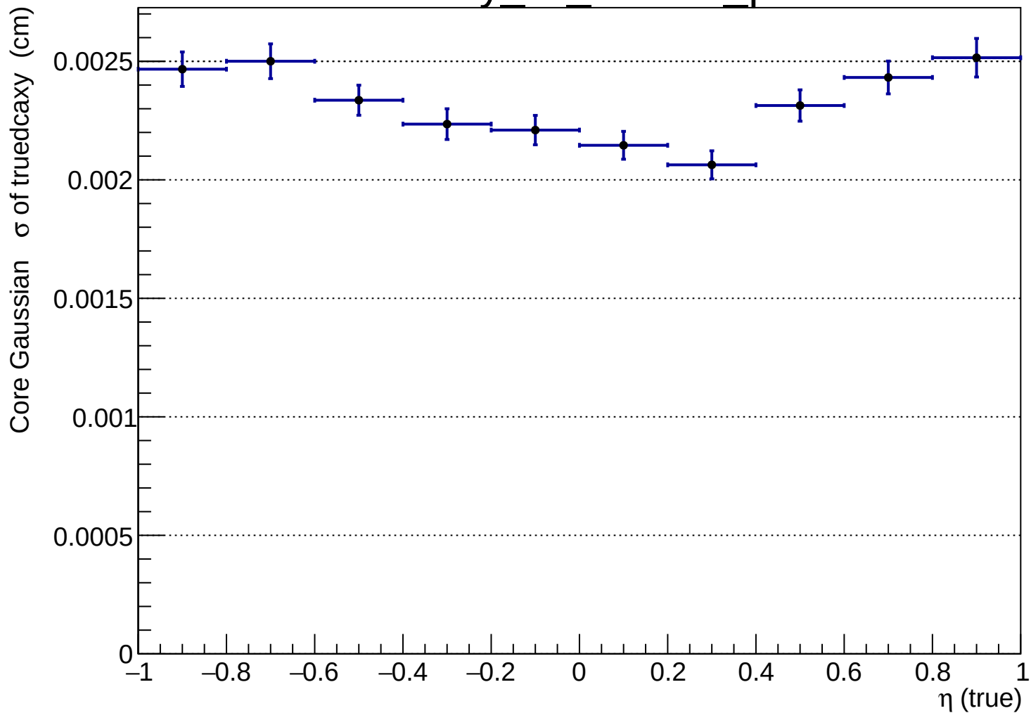
htruedcaxy_vs_etatruē
