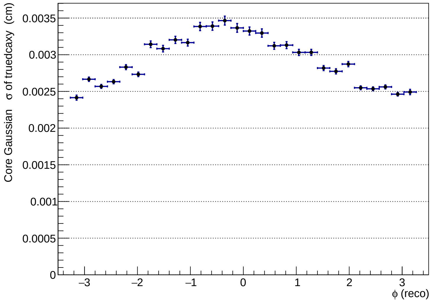
htruedcaxy_vs_phireco_pi+
