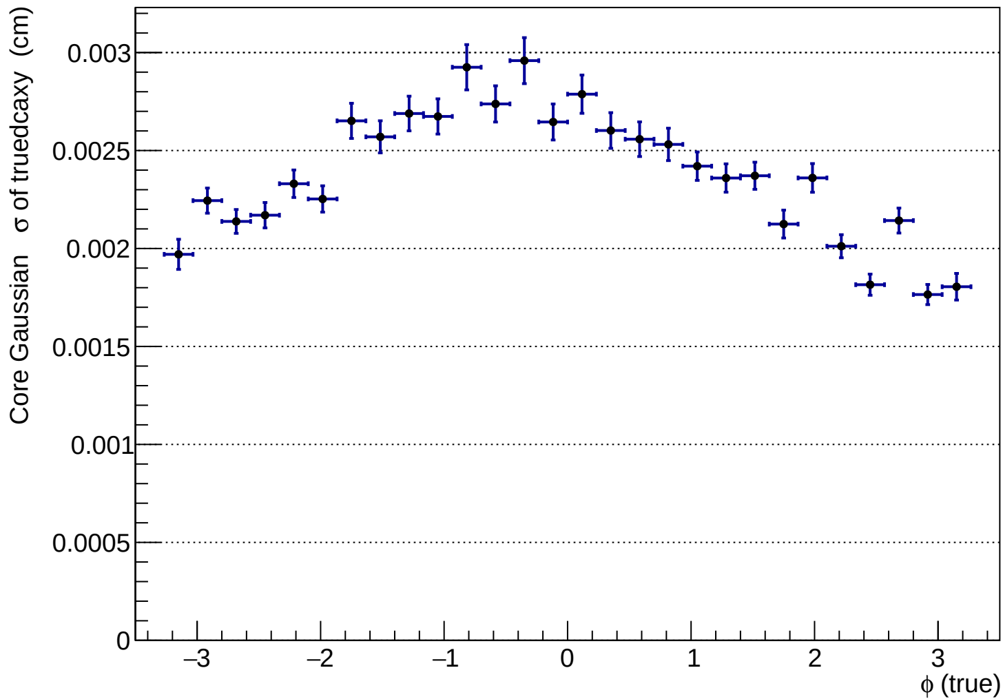
htruedcaxy_vs_phitru_K+
