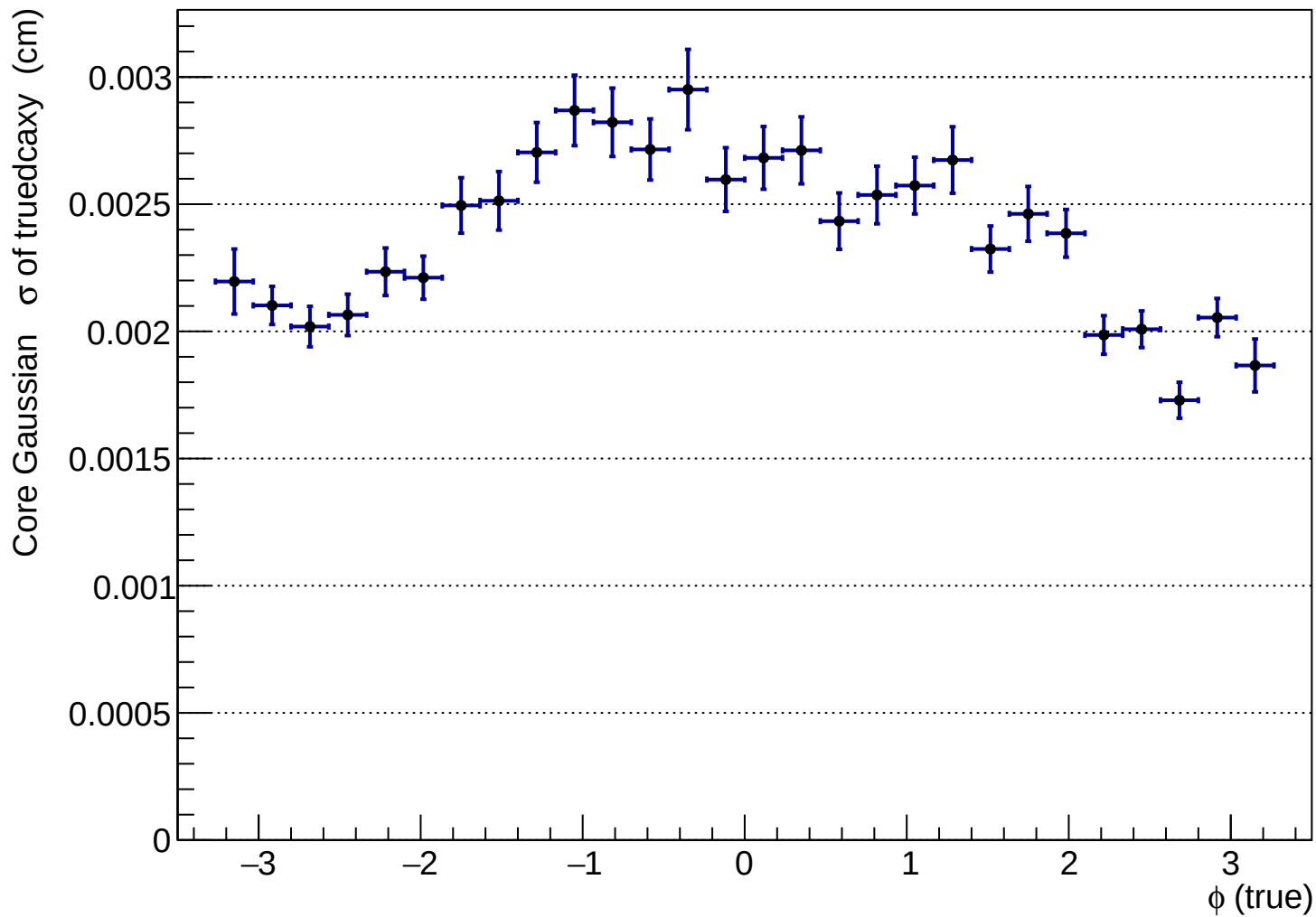
htruedcaxy_vs_phitruue_p
