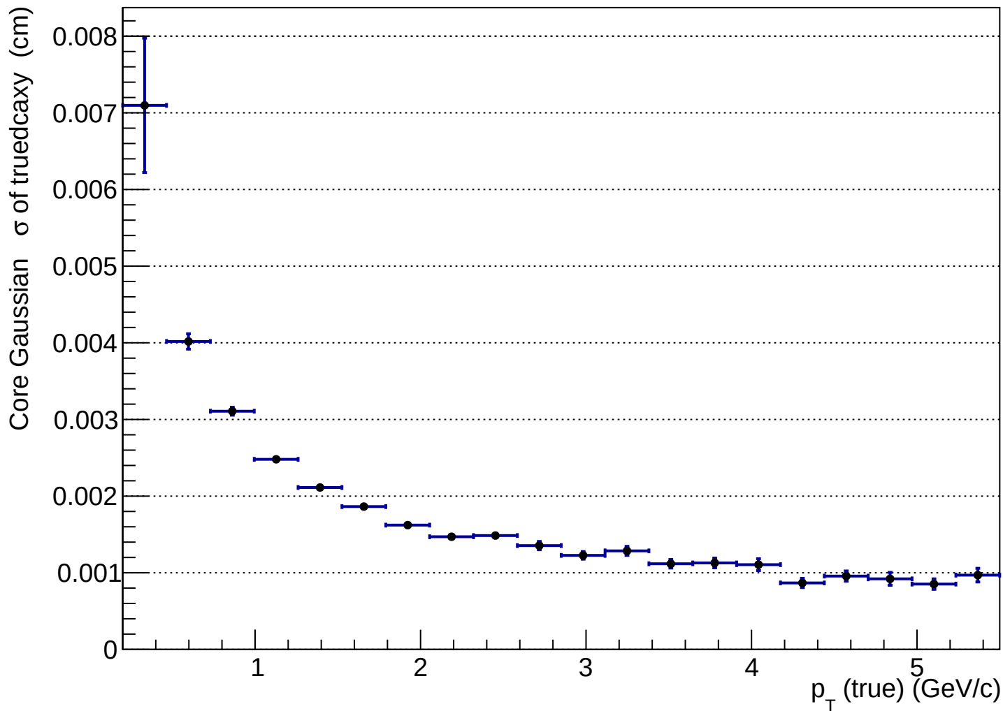
htruedcaxy_vs_pttrue_K+
