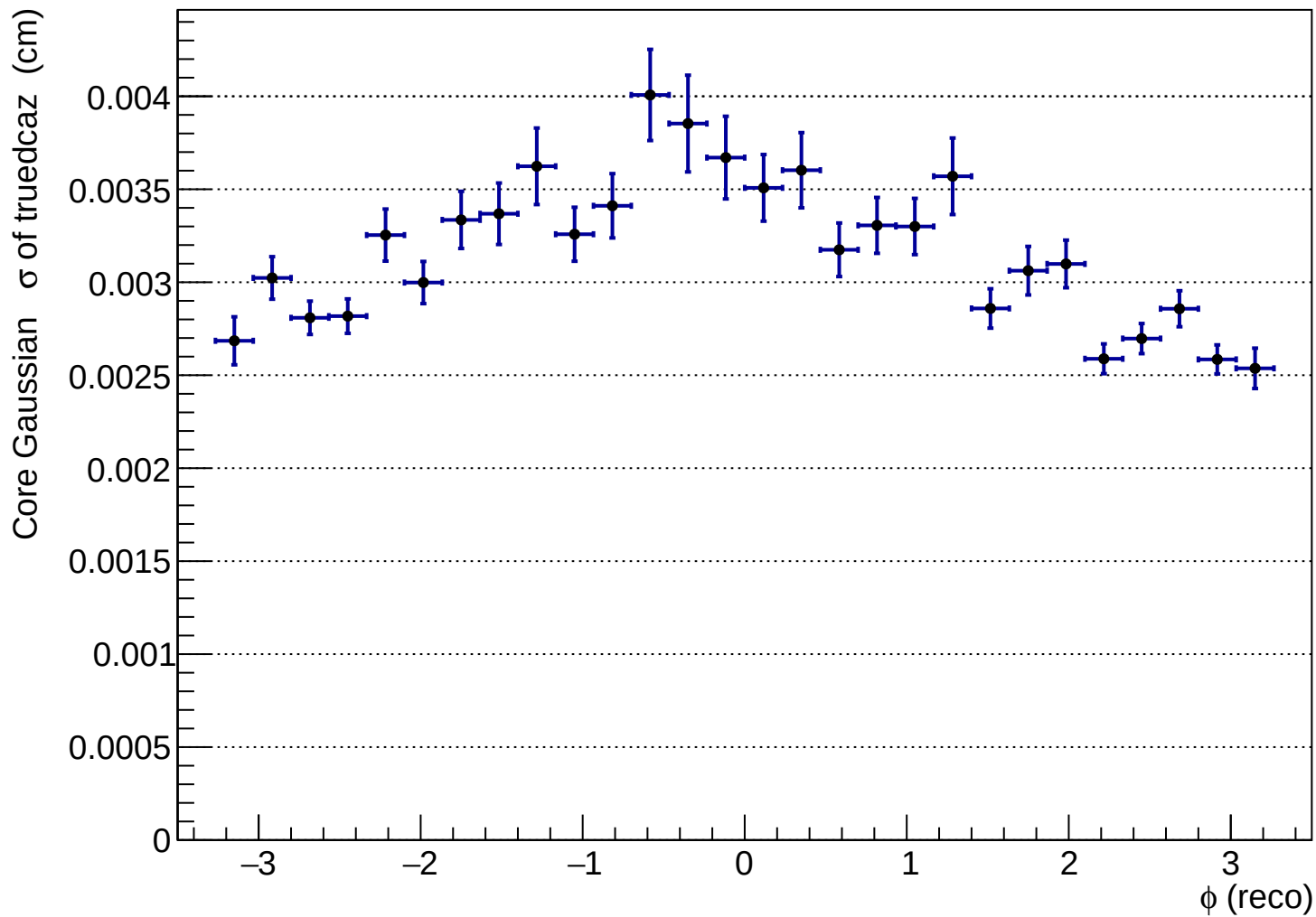
htruedcaz_vs_phireco_K+
