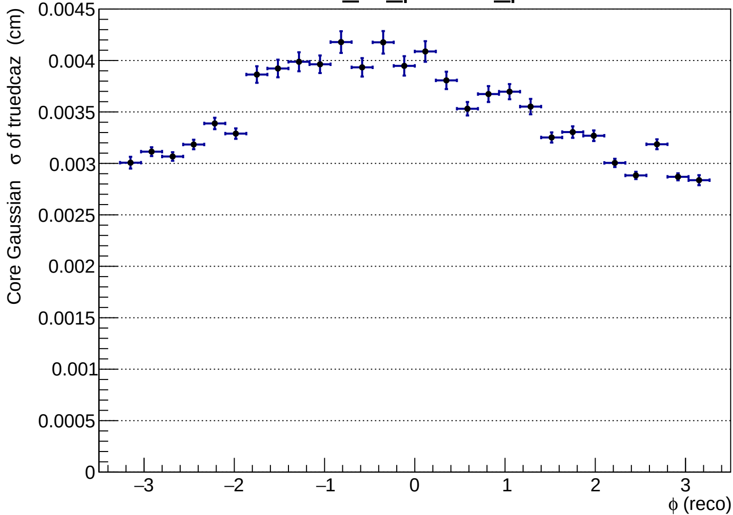
htruedcaz_vs_phireco_pi-
