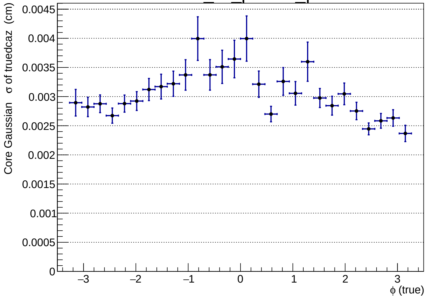
htruedcaz_vs_phitruue_p̄
