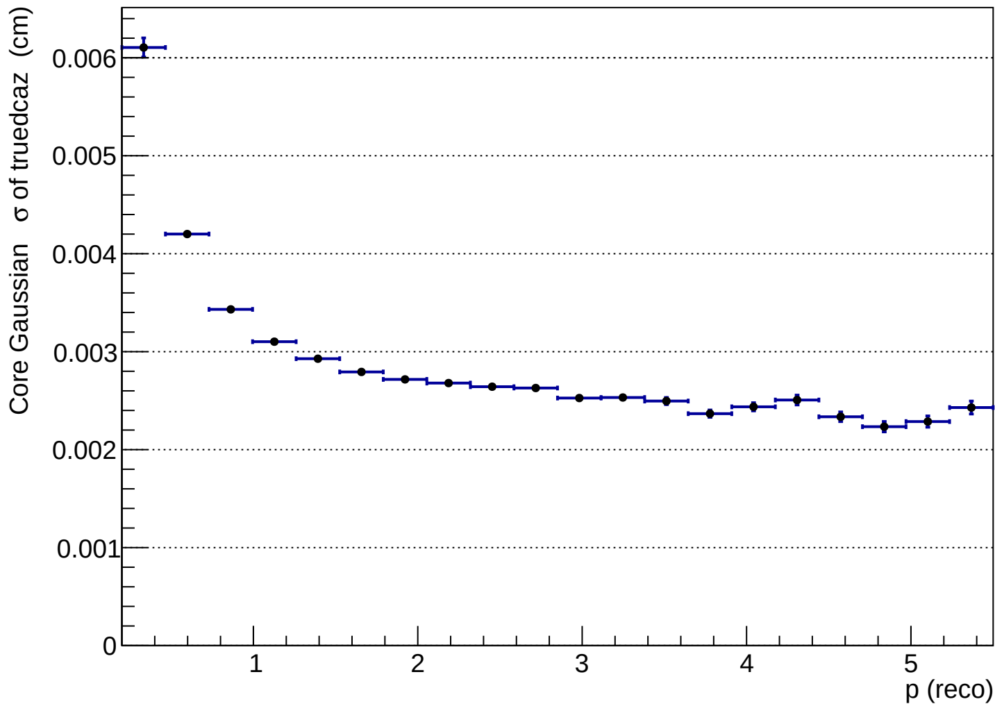
htruedcaz_vs_preco
