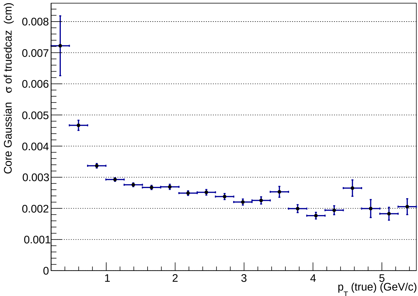
htruedcaz_vs_pttrue_K+
