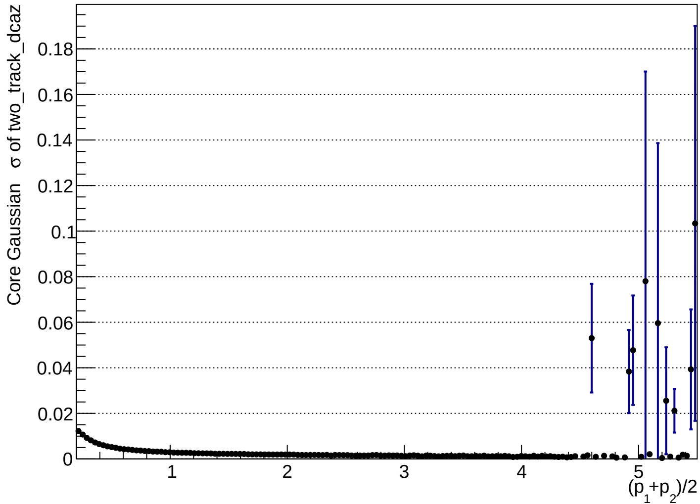
Two track dcaz vs p
