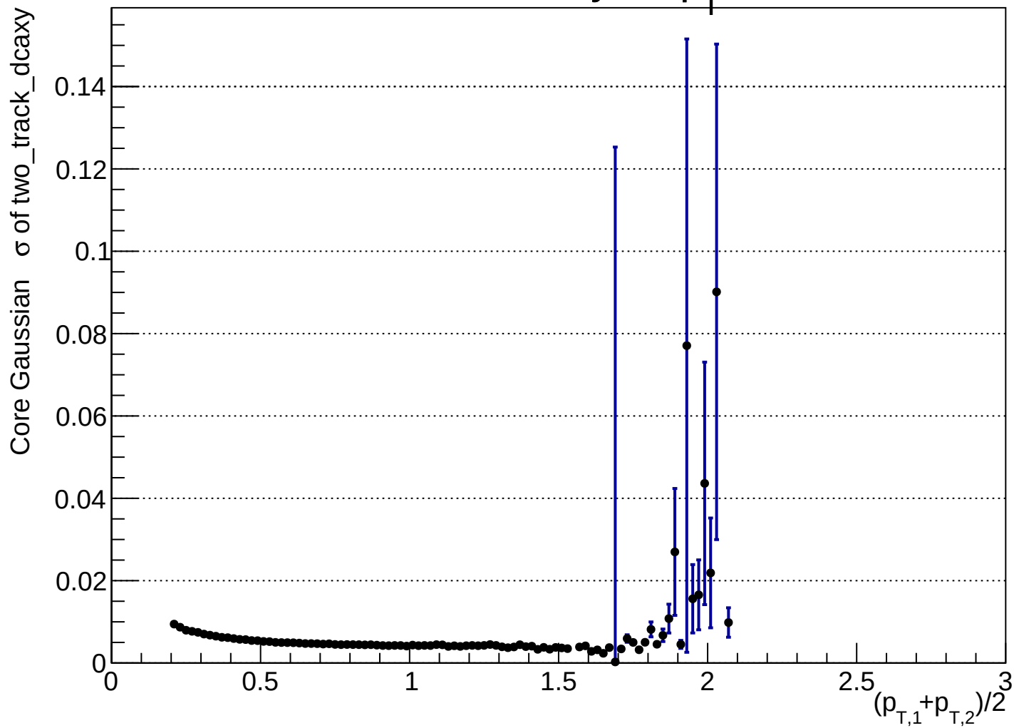
Two track dca xy vs p_T
