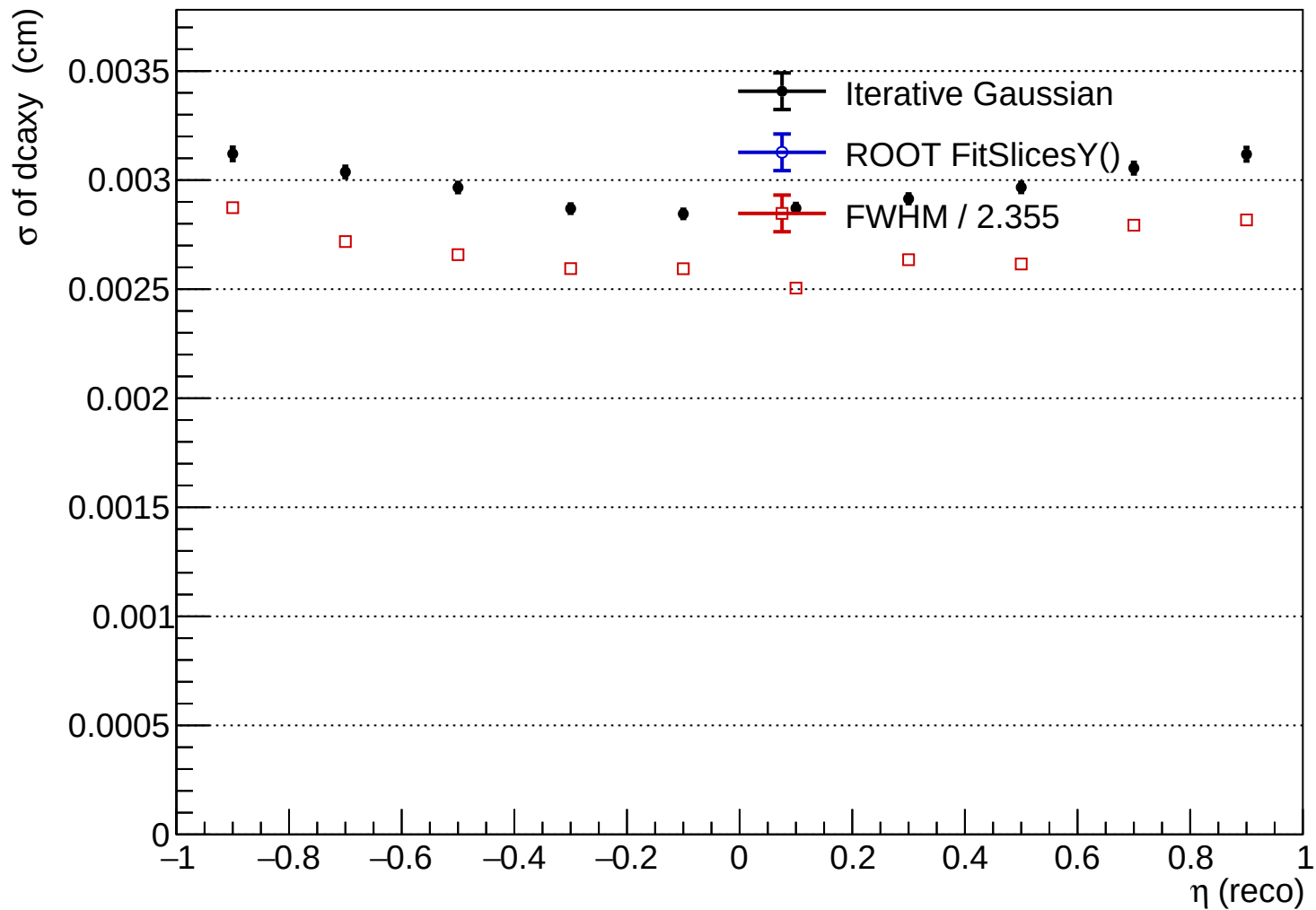
hdcaxy_vs_eta_reco_pi+
