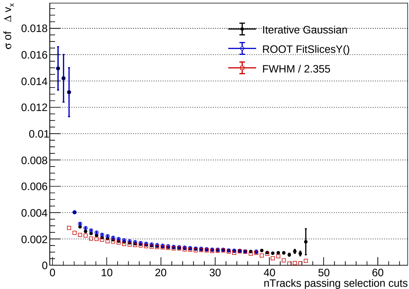
\Delta v_x vs nTracks
