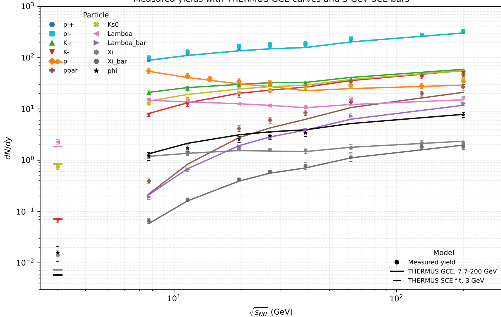
Measured yields with THERMUS GCE curves and 3 GeV SCE bars
